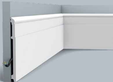
SX156 HIGH HEELS 200 x 20,2 x 1,6 cm Duopolymer® Designed by Xavier Donck
